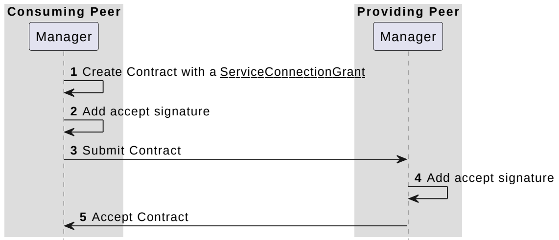
Figure 5 Connecting to a Service
