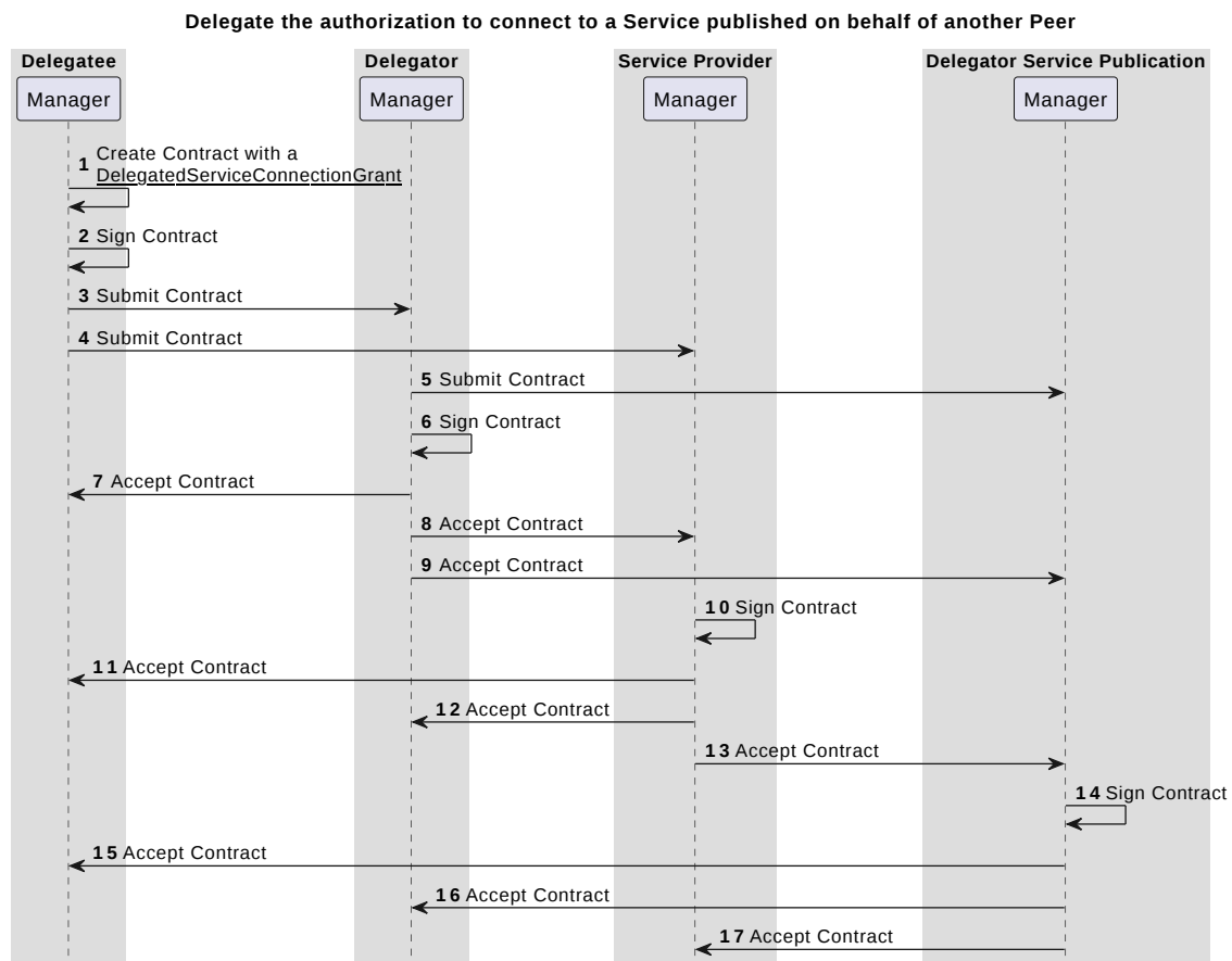
Figure 8 Delegate a connection to a Service that is offered on behalf of another Peer
